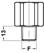
23M - 1/4-18 NPT
